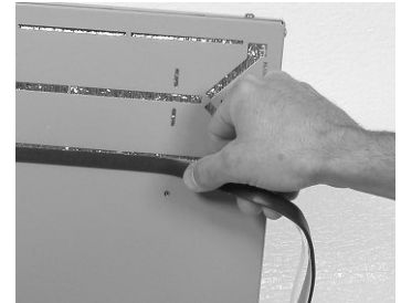
figure 2.2h - Apply plenum seal tape all around both openings on the back of the unit.
